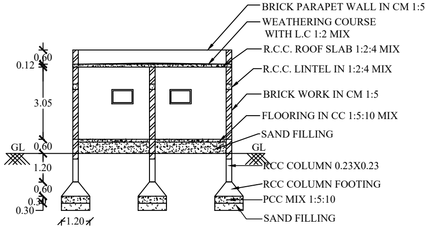
SECTION OF "AB"
